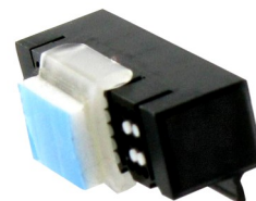
ADHESIVE CLIP 8mm(W) x 7mm (H) Holds modules with or without frame. Ideal on glasses or watches. Does not include module. TX-500420
