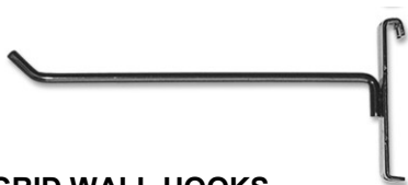
GRID WALL HOOKS Black 100mm GW-BH4 Black 150mm GW-BH6 Black 200mm GW-BH8 Black 250mm GW-BH10
